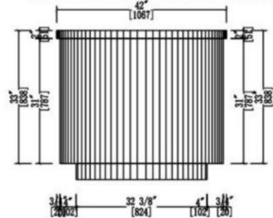
(E) ELEVATION
