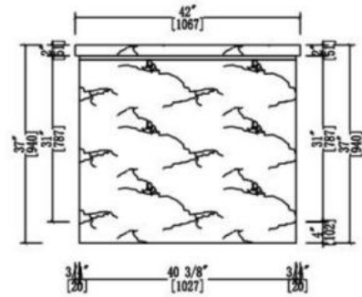
(C) ELEVATION
