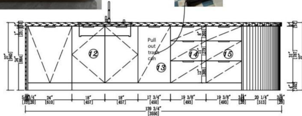
(B) ELEVATION
